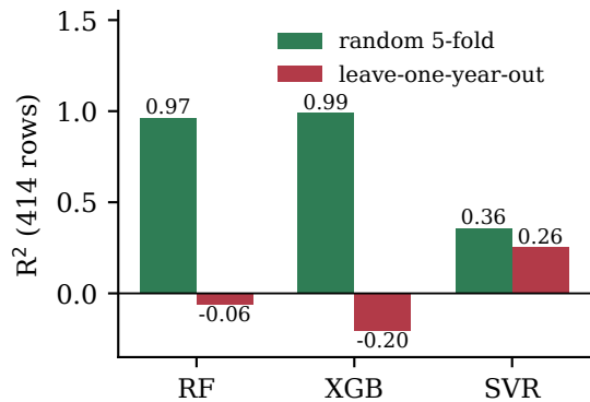
(a) Same rows, two protocols
